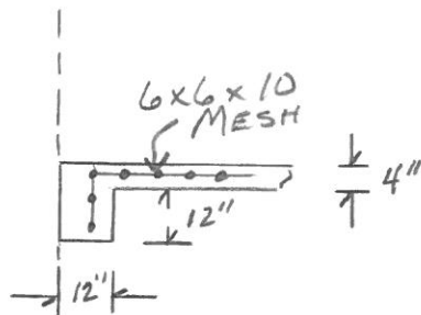
FLOOR DETAIL
